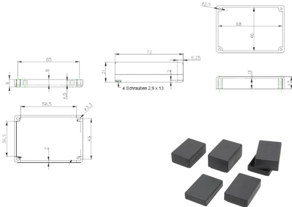
Foto zeigt KG15M – KG41M Photo shows KG15M – KG41M
